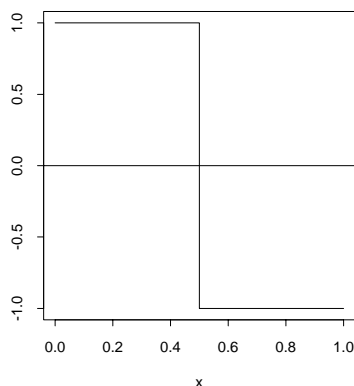
Figure 3: Haar wavelet
